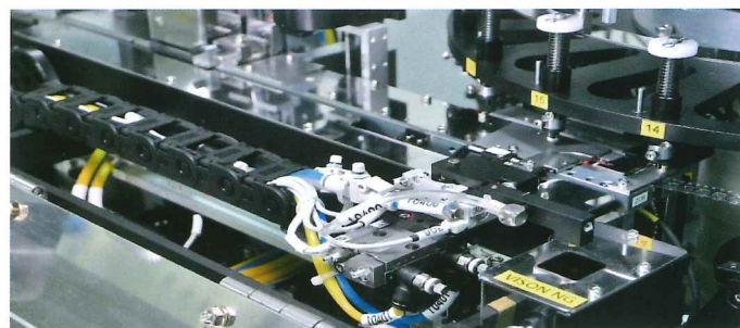
良品補料站 Auto good product replenishment mechanism
